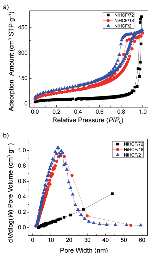
Figure 2. N_2 –196 °C isotherms of the NiHCF/ t series (a) and corresponding BJH pore-size distribution (PSD) curves (b).
